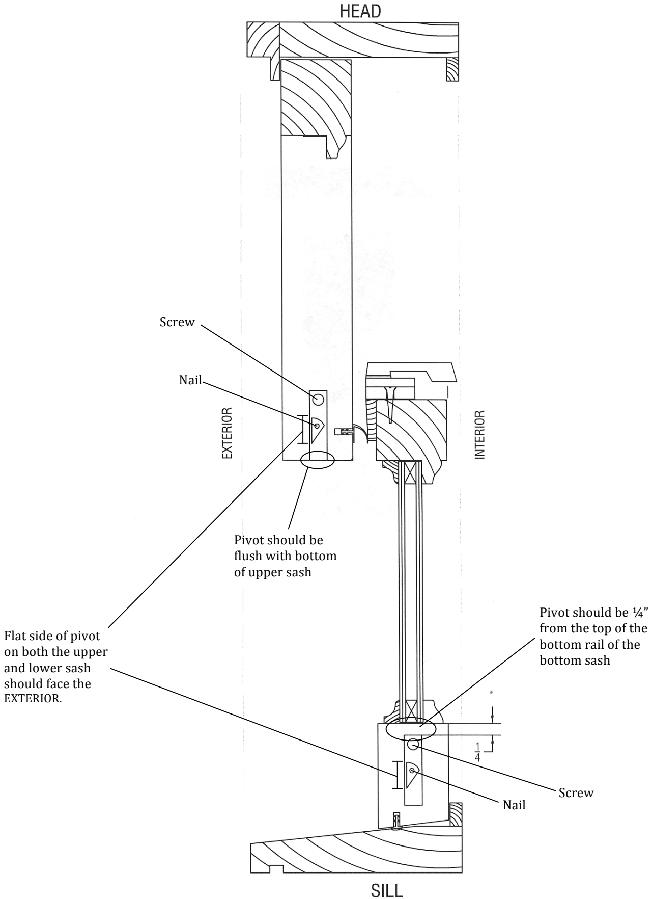
VERTICAL SECTION VIEW
